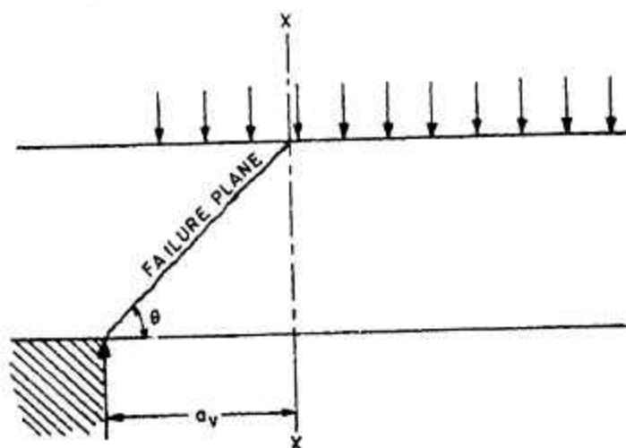
FIG. 24 SHEAR FAILURE NEAR SUPPORTS
