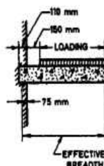
FIG. 19 LOADING ON STAIRS BUILT INTO WALLS
