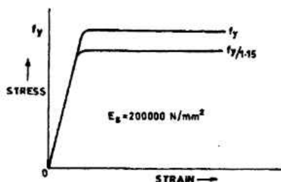
23B STEEL BAR WITH DEFINITE YIELD POINT
