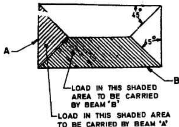
FIG. 7 LOAD CARRIED BY SUPPORTING BEAMS
