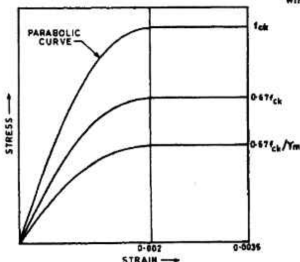
FIG. 21 STRESS-STRAIN CURVE FOR CONCRETE
