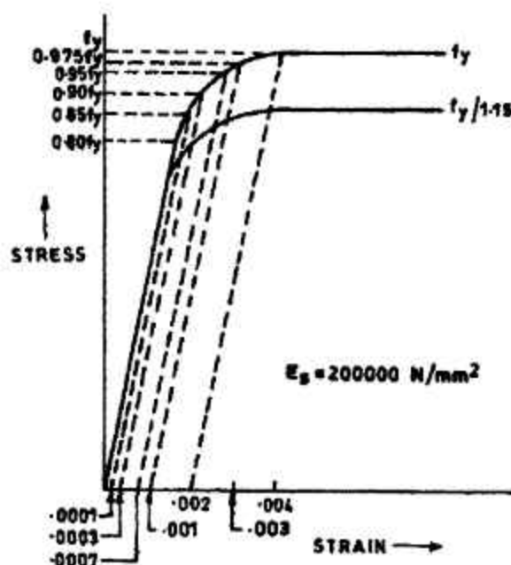
23A Cold Worked Deformed Bar
